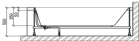
AA SECTION
