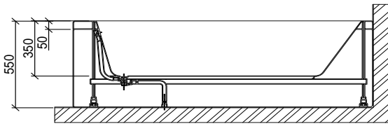
AA SECTION
